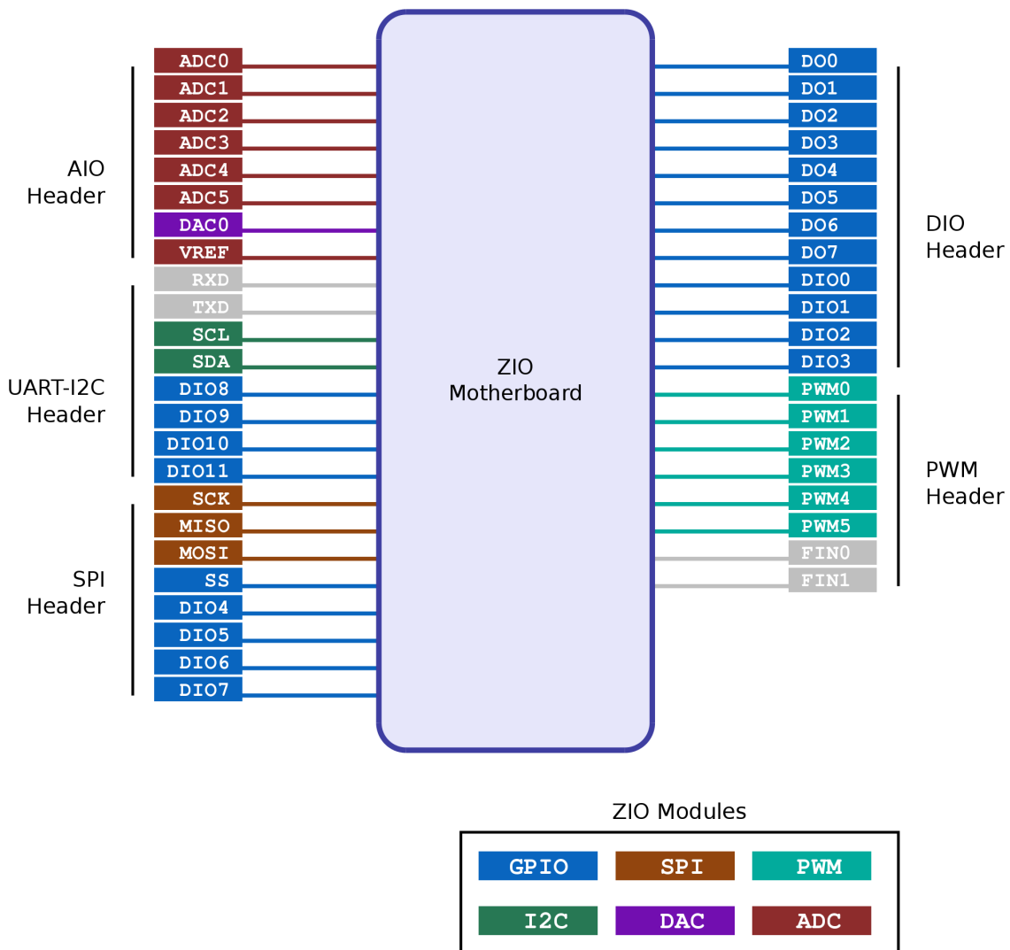
Figure 1.1. ZIO Modules and Signals
