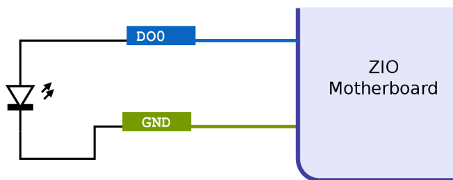
Figure 2.1. LED Circuit
