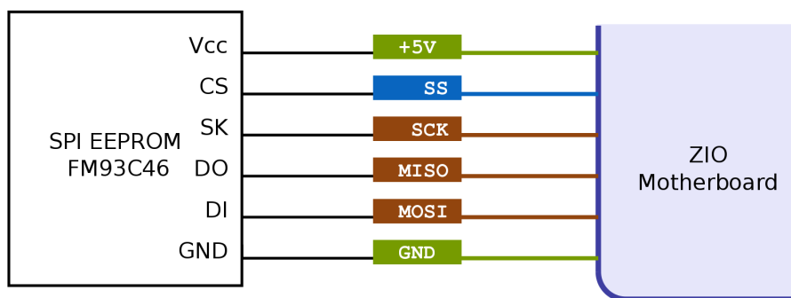
Figure 2.5. SPI EEPROM Circuit
